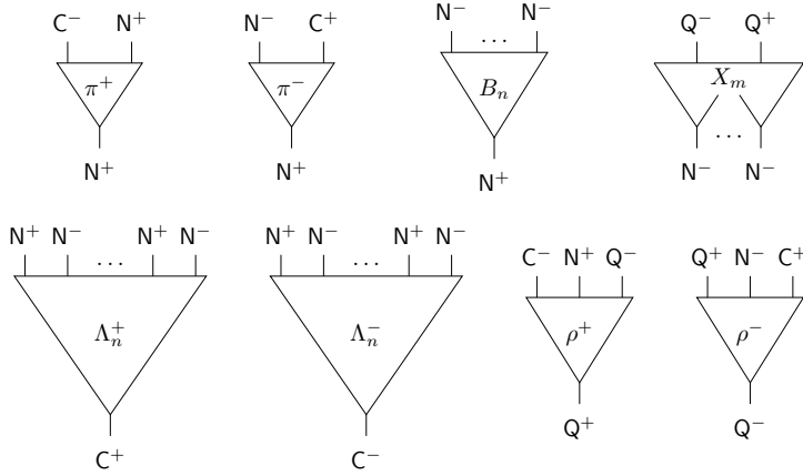
Figure 5.4: The alphabet of \mathcal{F}_\infty
