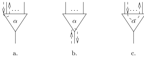
Figure 2.1: a,b. Bouncing paths. c. Twisting path.
