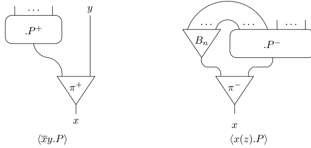
Figure 5.6: The construction of .P^\epsilon from a net of the form \langle P \rangle .
