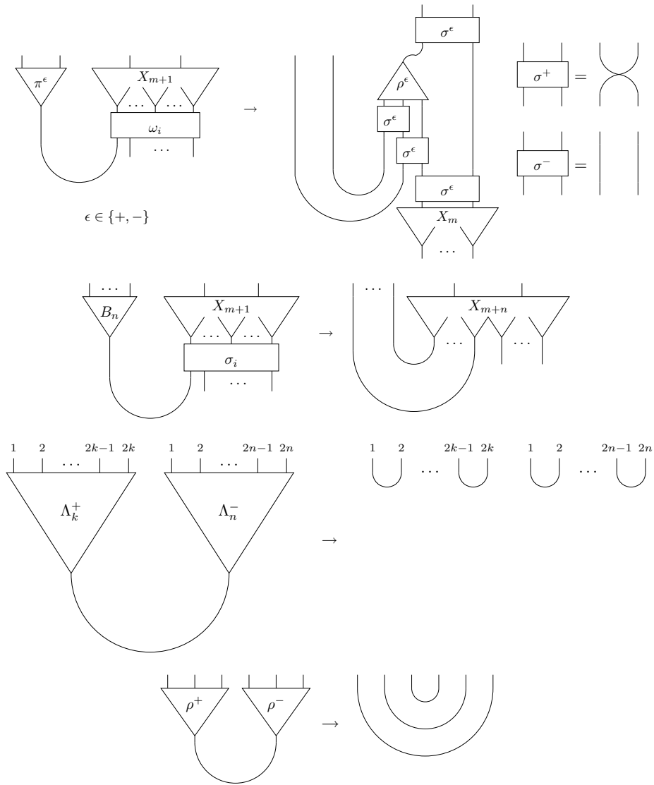
Figure 5.5: The rules of \mathcal{F}_\infty
