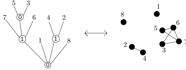
FIGURE 3. Left: A labeled cotree t with 8 leaves. Right: The associated labeled cograph \text{Cograp}(t) of size 8.
