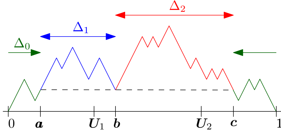
FIGURE 2. A stylized version of a Brownian excursion and the corresponding \mathbf{a}, \mathbf{b}, \mathbf{c}, \Delta_0, \Delta_1, \Delta_2 .
