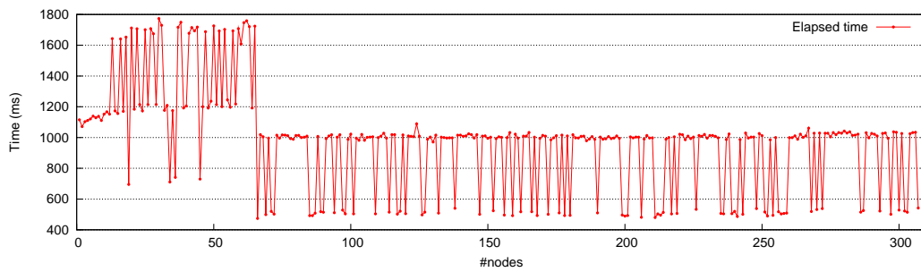
Fig. 6. Elapsed time for sequential registrations of Free-Pastry services
