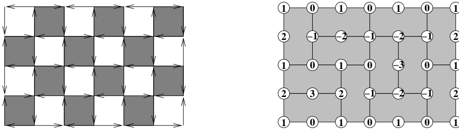
FIGURE 2. A set of chessboard-like colored cells and the directed edges of the associated graph (left). A domino tiling \mathcal{T} of this set of cells and a corresponding function h_{\mathcal{T}} (right).
