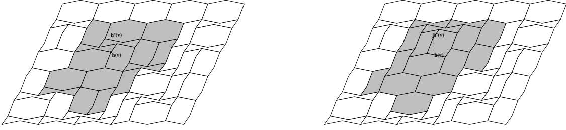
FIGURE 6. Three-dimensional viewpoint of a height function h , with the shaded dominoes being those which have vertices in the set S_{v, h'(v), h(v)} (left). Here, there is a finite number of shaded dominoes: any other tiling over the same set of cells can thus be obtained by performing a finite number of flips. In particular, this holds for the restriction of the pyramid \hat{h}_{v, h'(v)} to S_{v, h'(v), h(v)} (the shaded dominoes, right). This transforms h into a height function that is equal to h' in v .
