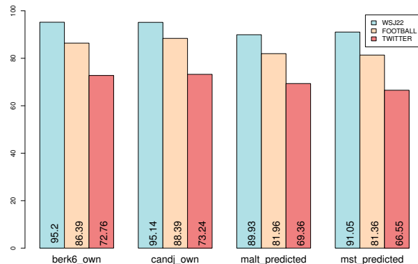
Figure 1: F-scores for nsubj
