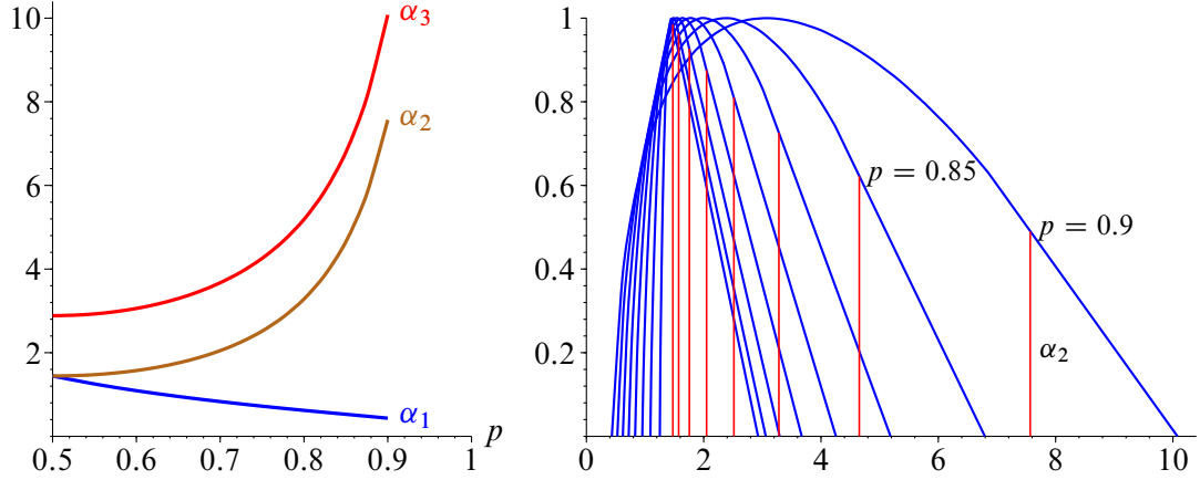
Figure 2: Left: Plot of \alpha_1 , \alpha_2 , and \alpha_3 (defined in (5)) as functions of p . Right: The (non-zero) limiting order of \log \mu_{n,k} / \log n plotted against \alpha = \lim_n k / \log n for p = 0.55, 0.6, \dots, 0.9 (the spans of the curves increase as p grows). The vertical lines represent the positions of \alpha_2 (to the right of which the curves are straight lines); see (4).
