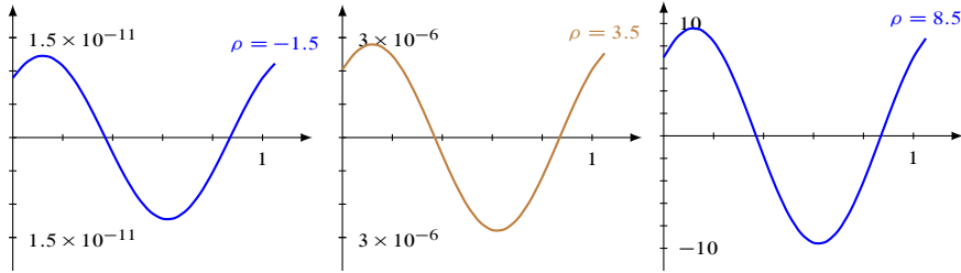
Figure 4: The fluctuating part around the mean of the periodic function G_1(\rho; x) for \rho \in \{-1.5, 3.5, 8.5\} and x \in [0, 1] . The amplitude increases as \rho grows.
