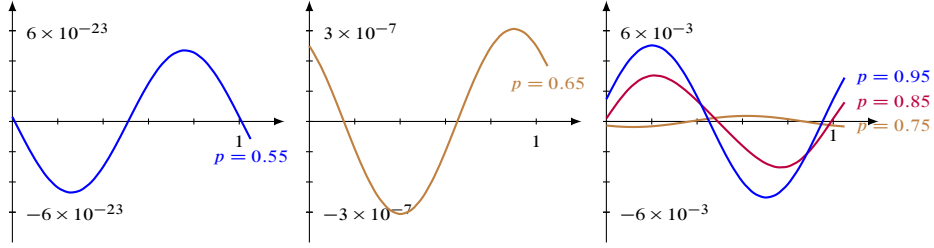
Figure 3: The fluctuating part around the mean of the periodic function G_1(-1; x) for p = 0.55, 0.65, \dots, 0.95 and for x in the unit interval; its amplitude tends to zero when p \rightarrow 0.5^+ .
