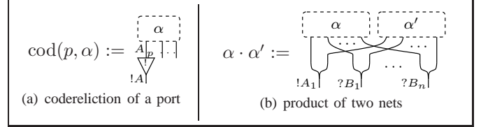
Figure 3: codeleriction and product of simple nets.
