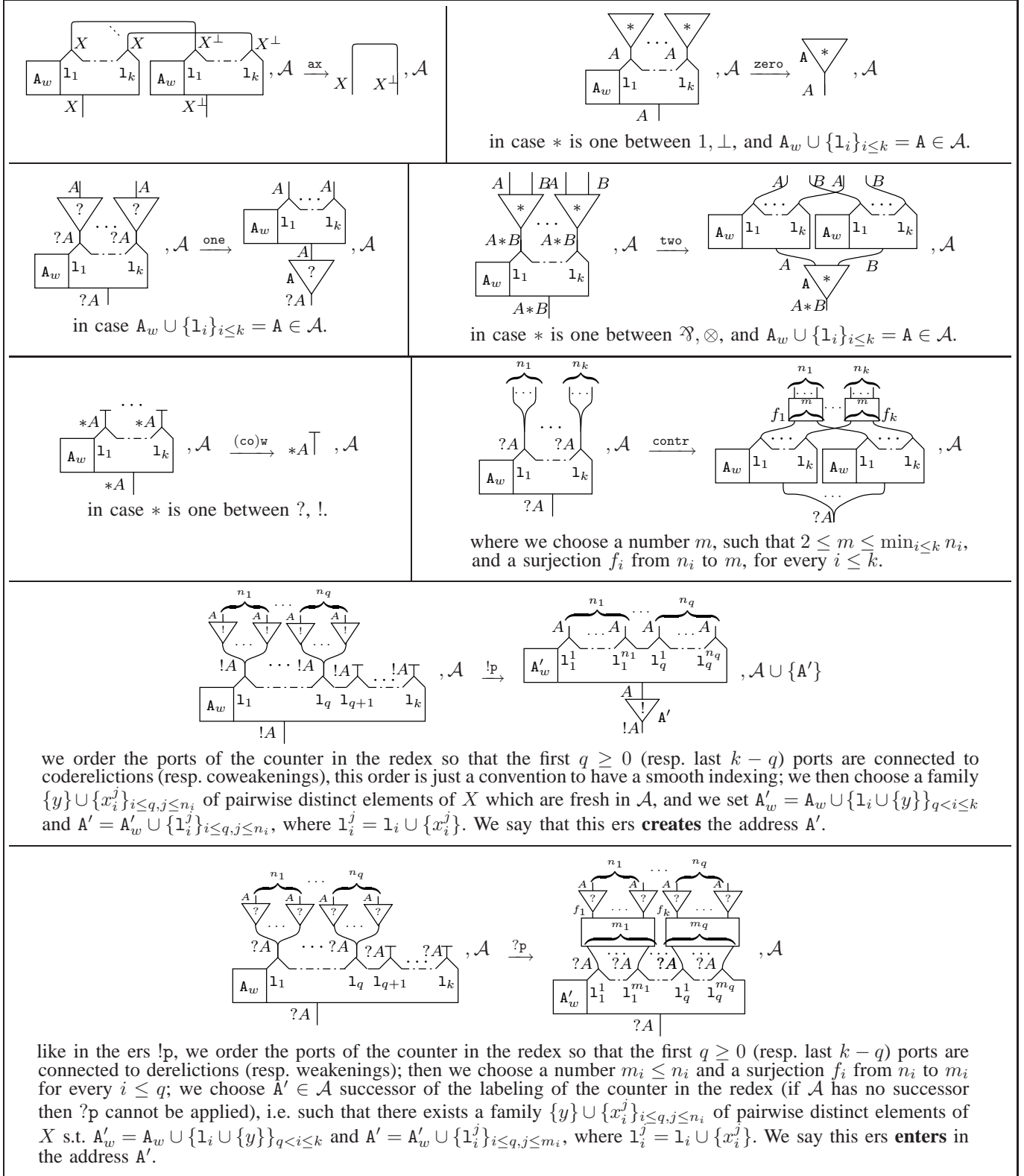
Figure 9: the elementary reduction steps (ers for short) of merging reduction; the net at left of an ers is the redex , the one at right is the contractum of the ers. In the ers contr, ?p , we present a bunch of contractions and wirings as a surjective function f from the auxiliary ports to the principal ones.
