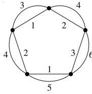
Figure 3: An example for which the natural greedy algorithm fails. The graph is a 2-uniform 5-cycle, and has chromatic edge strength \max\{\Delta, \lceil m/k \rceil\} = \max\{4, \lceil 10/2 \rceil\} = 5 . However, iteratively removing maximum matchings can yield a 6-coloring.
