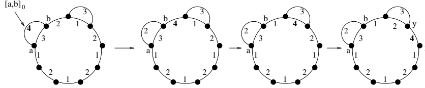
Figure 2: An illustration of the case \sigma \in C_a \cap C_b in the proof of Theorem 4, with s' = \chi' = 3 . Again, [a, b]_0 is the only edge colored with color s' + 1 = 4 , and \sigma = 3 .
