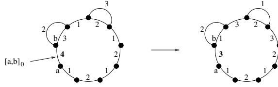
Figure 1: An illustration of the case \sigma \in C_b \setminus C_a in the proof of Theorem 4, on a multicycle G with s' = \chi' = 3 . The edge [a, b]_0 is the only edge colored with color s' + 1 = 4 . In this example, color \sigma = 3 and color \alpha \in C_a \setminus C_b is equal to 1.
