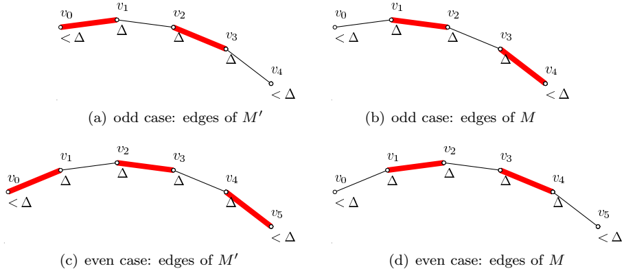
Figure 4: Illustration of the proof of Lemma 1.
