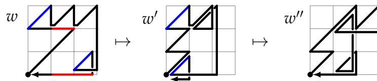
Figure 2: An example of the mapping w \mapsto w'' in the proof of Theorem 1.
