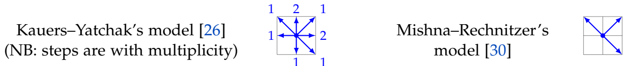
Figure 5: Forbidding some steps in the left (algebraic) model leads to the right (hyper-transcendental) model (as follows by the work of Singer and Hardouin [22]).
