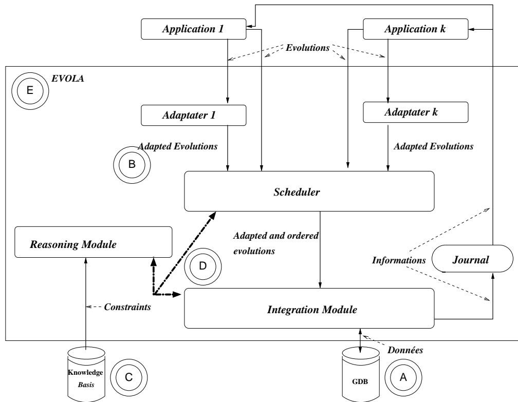
Figure 8: EVOLA architecture
