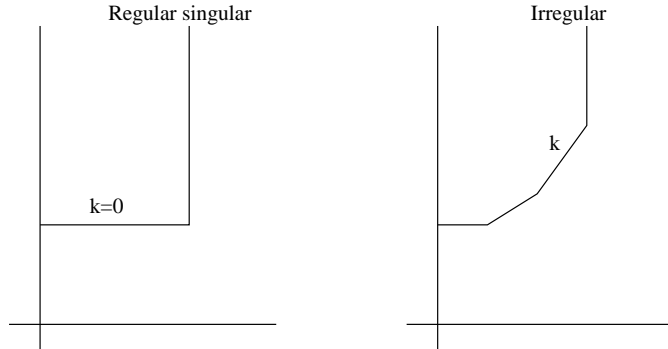
Figure 2.2: Newton polygons
