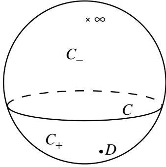
Figure 2.1: Birkhoff Decomposition
