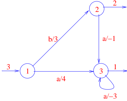
Figure 1: Automata with multiplicities
