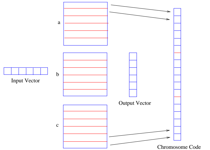
Figure 2: Chromosome code
