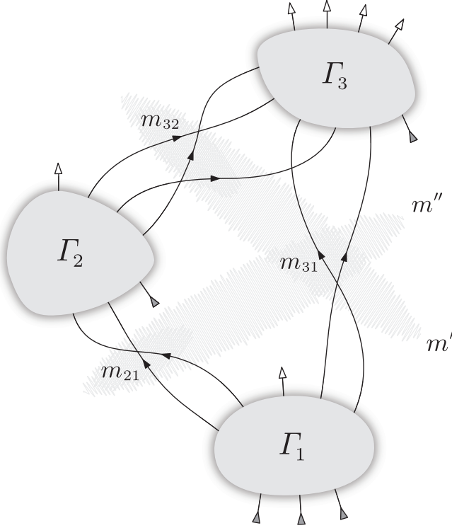
FIG. 4 Fine graining of the matchings m' \in \Gamma_3^- \triangleleft (\Gamma_2 \overset{m_{21}}{\triangleleft} \Gamma_1)^+ and m'' \in (\Gamma_3 \overset{m_{32}}{\triangleleft} \Gamma_2)^- \triangleleft \Gamma_1^+ used in the proof of associativity of multiplication.
