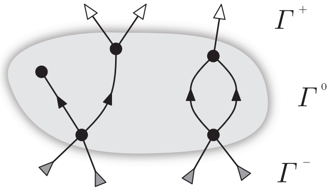
FIG. 1 An example of a Heisenberg–Weyl diagram with three distinguished characteristic sorts of lines: the inner ones |\Gamma^0| = 4 , the incoming lines |\Gamma^-| = 4 and outgoing lines |\Gamma^+| = 3 .
