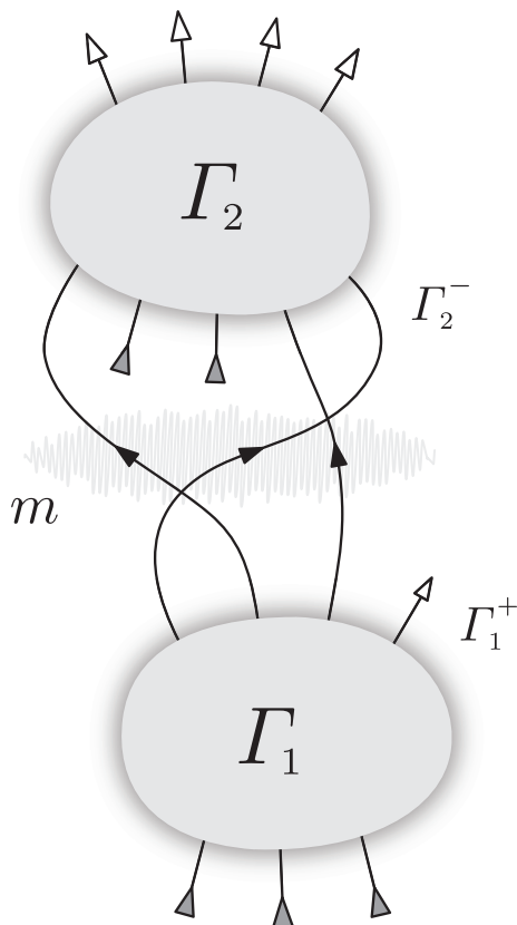
FIG. 2 Composition of two diagrams \Gamma_2 \overset{m}{\llcorner} \Gamma_1 according to the matching m \in \Gamma_2^- \llcorner \Gamma_1^+ consisting of three connections.
