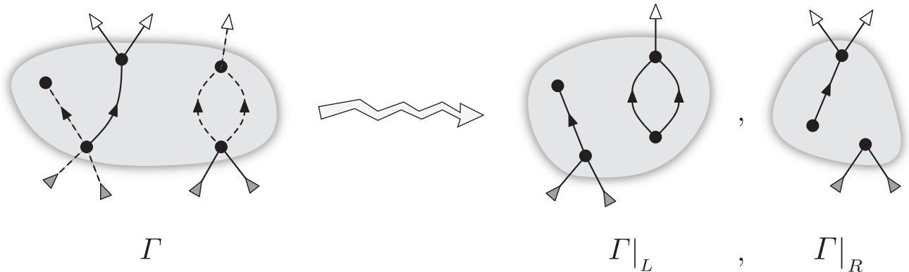
FIG. 3 An example of diagram decomposition \Gamma \rightsquigarrow (\Gamma|_L, \Gamma|_R) . The choice of edges L \subset E_\Gamma inducing the diagram \Gamma|_L is depicted on the left diagram as dashed lines.
