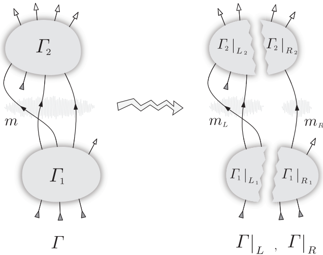
FIG. 6 Decompositions of a composite diagram \Gamma = \Gamma_2 \overset{m}{\triangleleft} \Gamma_1 for some m \in \Gamma_2 \triangleleft \Gamma_1 used in the proof of condition (4).
