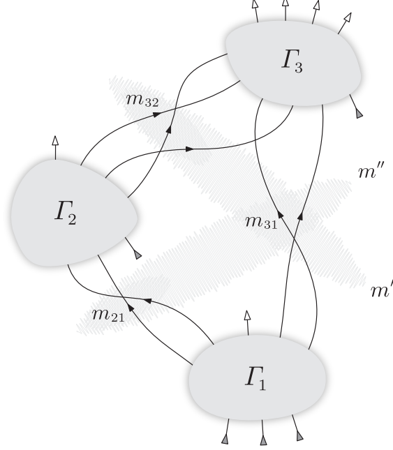
Figure 4: Fine graining of the matchings m' \in \Gamma_3^- \triangleleft (\Gamma_2 \xrightarrow{m_{21}} \Gamma_1)^+ and m'' \in (\Gamma_3 \xrightarrow{m_{32}} \Gamma_2)^- \triangleleft \Gamma_1^+ used in the proof of associativity of multiplication.
