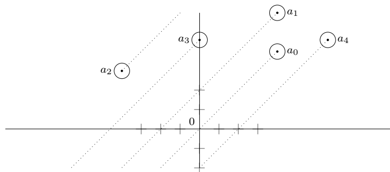
FIGURE 5 – Ouvert \Omega .
